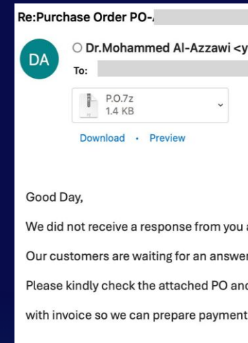
PHISHING
